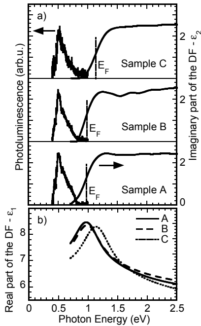
Figure 2 a) PL spectra at T = 10 \text{ K} and imaginary parts of the DF at RT for c-InN. The PL curves have been normalized to equal amplitude for the sake of clarity, the transition energies at the Fermi wave vector are indicated by E_F . The real parts of the DF are shown in b).
