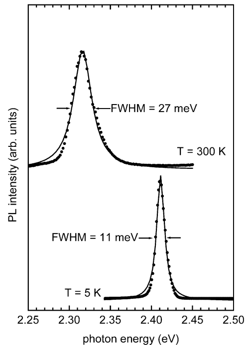
Fig. 2. Photoluminescence measurements of the quantum wells before mirror deposition at 5 K and at room temperature (dots). The lines were fitted with Lorentzian functions. The FWHM at 5 K is 11 and 27 meV at room temperature, respectively.
